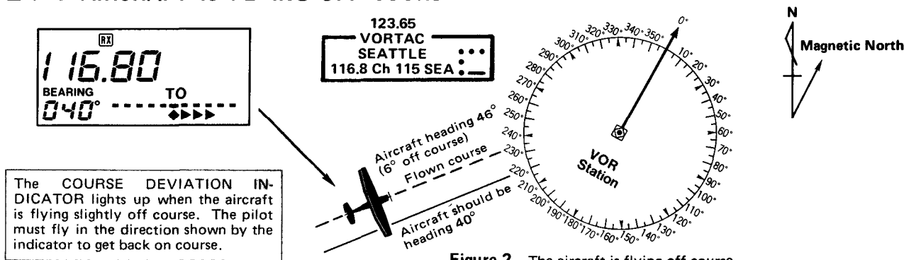
Figure 2 The aircraft is flying off course
