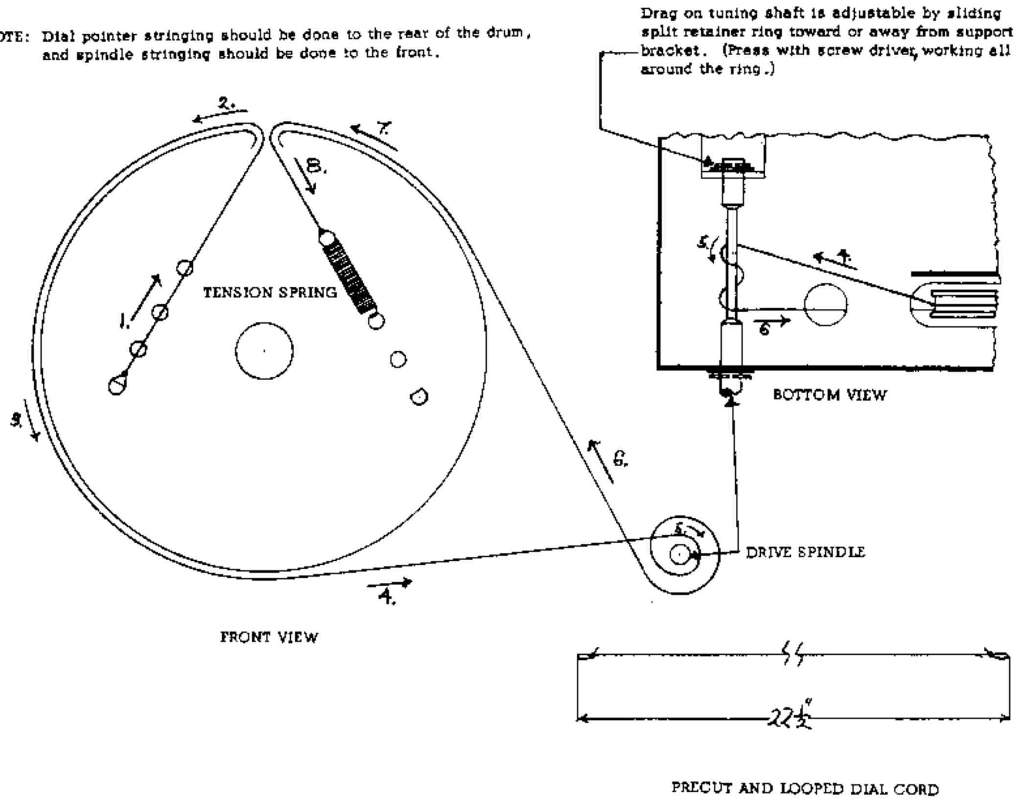
FIG. 1 DIAL POINTER STRINGING
